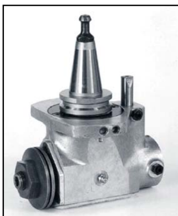
C-Axis Saw Aggregate ISO30
